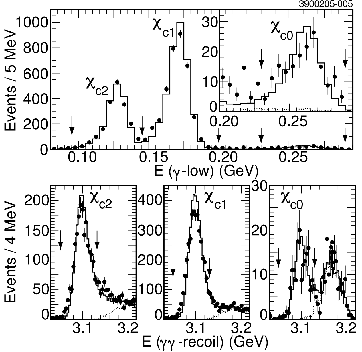
FIG. 4: For \psi(2S) \rightarrow \gamma\chi_{cJ} , \chi_{cJ} \rightarrow \gamma J/\psi , J/\psi \rightarrow \ell^+\ell^- candidate events in the \psi(2S) data (solid circles) and MC simulation of signal (solid line), the distribution of the energy of the second most energetic photon, E_{\gamma\text{-low}} , (top), and the two-photon recoil mass (bottom). The arrows indicate nominal cut values. The inset offers a close-up of the \chi_{c0} region. The broken lines represent \pi^0\pi^0 J/\psi MC.
