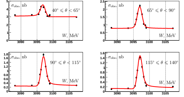
Figure 4: Fits to experimental data for the process e^+e^- \rightarrow e^+e^- in the J/\psi energy range for four angular ranges.
