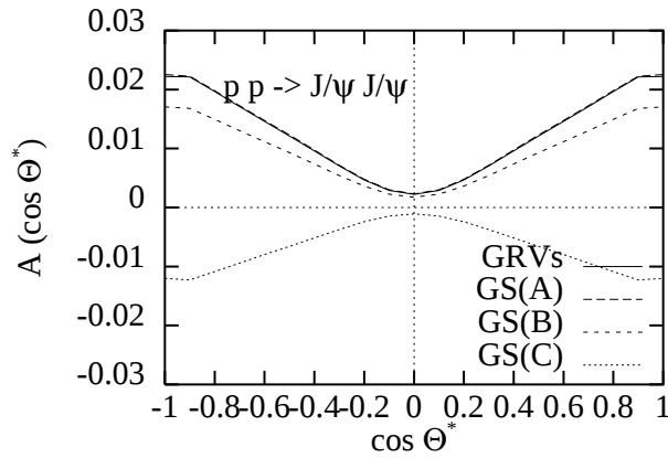
Figure 2: Expected asymmetry in the single polarized mode of HERA- \vec{N} .
