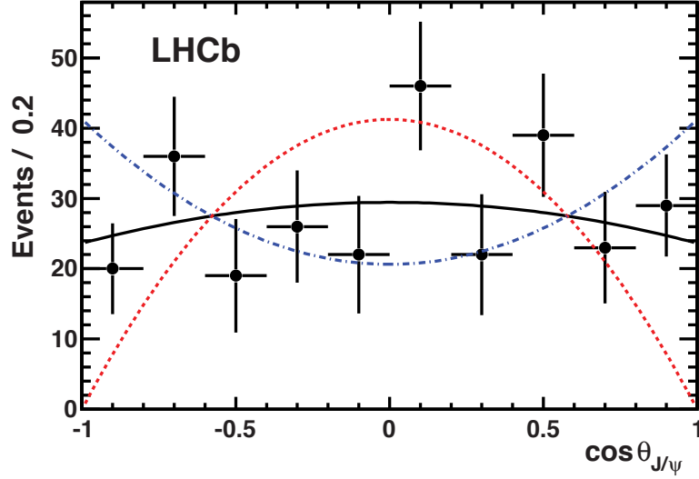
Figure 5: Distribution of \cos \theta_{J/\psi} for \overline{B}_s^0 \rightarrow J/\psi f_2' decays. The background and non-resonant K^+K^- components have been subtracted, and the data have been corrected for acceptance. The fit to Eq. 1 is shown by the solid line. Note that for pure S-wave the distribution would be \sin^2 \theta_{J/\psi} ( p = 0 ), shown as the dotted curve, while for pure helicity 1 ( p = 1 ) the data would be described by the dot-dashed curve.
