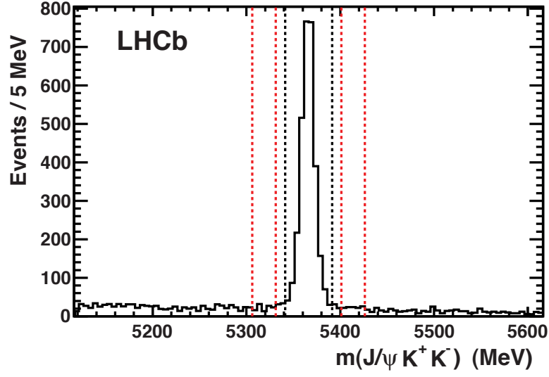
Figure 1: Invariant mass of J/\psi K^+ K^- combinations. The vertical lines indicate the signal and sideband regions.
